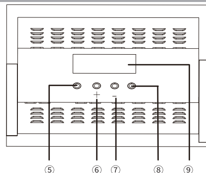
Fig.5 HL-180 Top view
