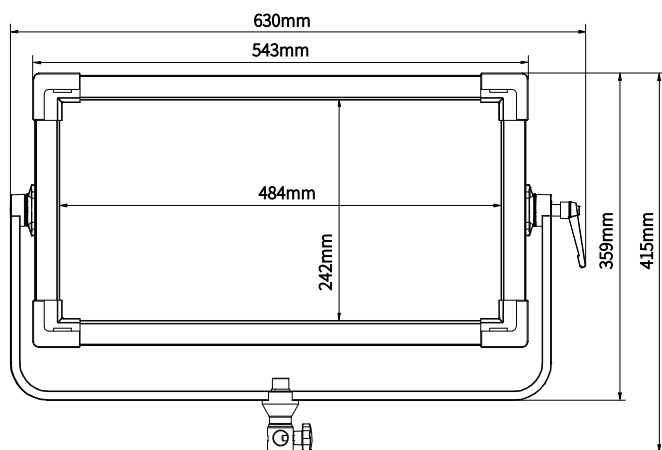
Fig.1 PL-S150D Dimension (Front view)
